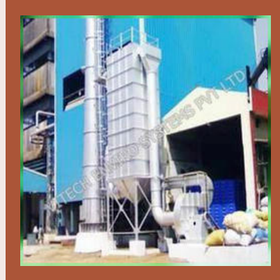
Bag Filter Dust Collector
